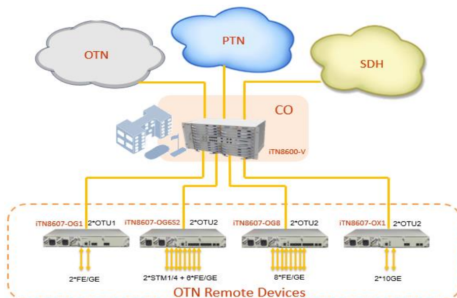
Figure 2: OTN Leased Line Application
